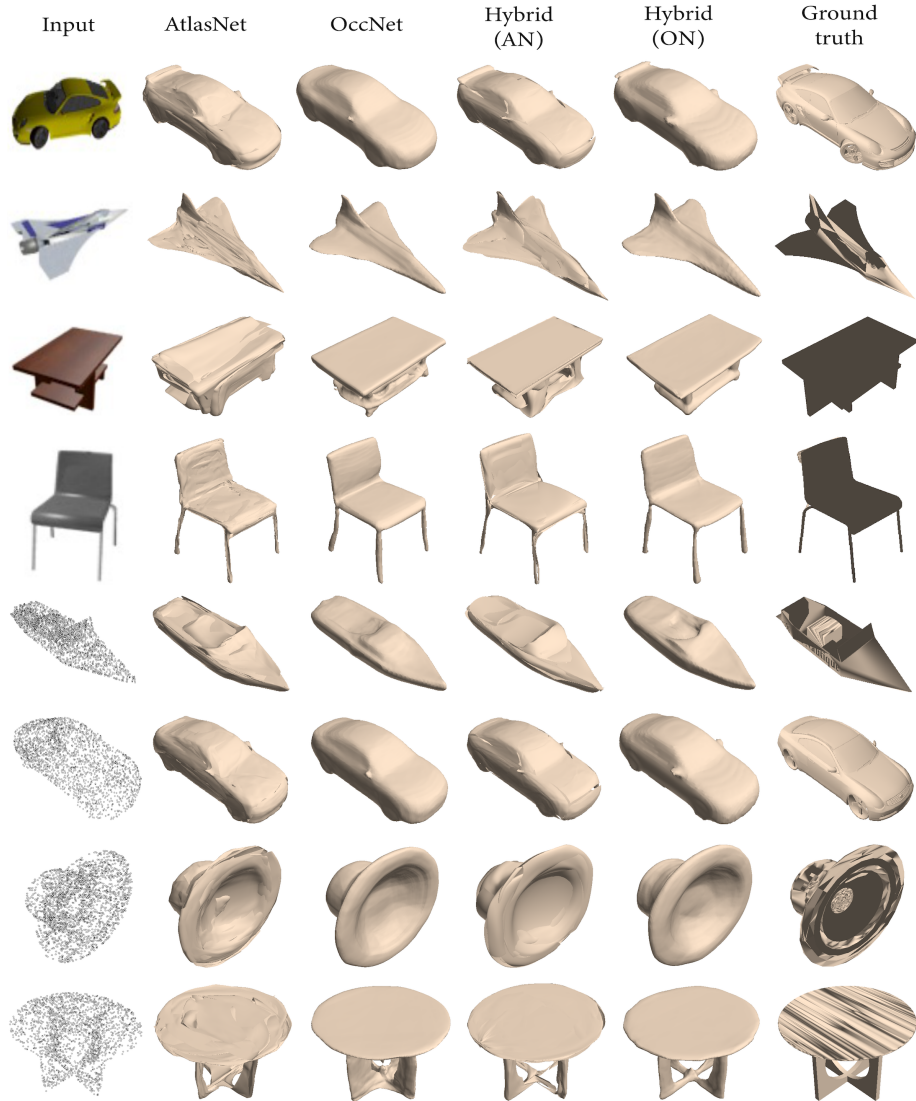
Fig. 1. Random results on reconstructing surfaces from images and point clouds.
